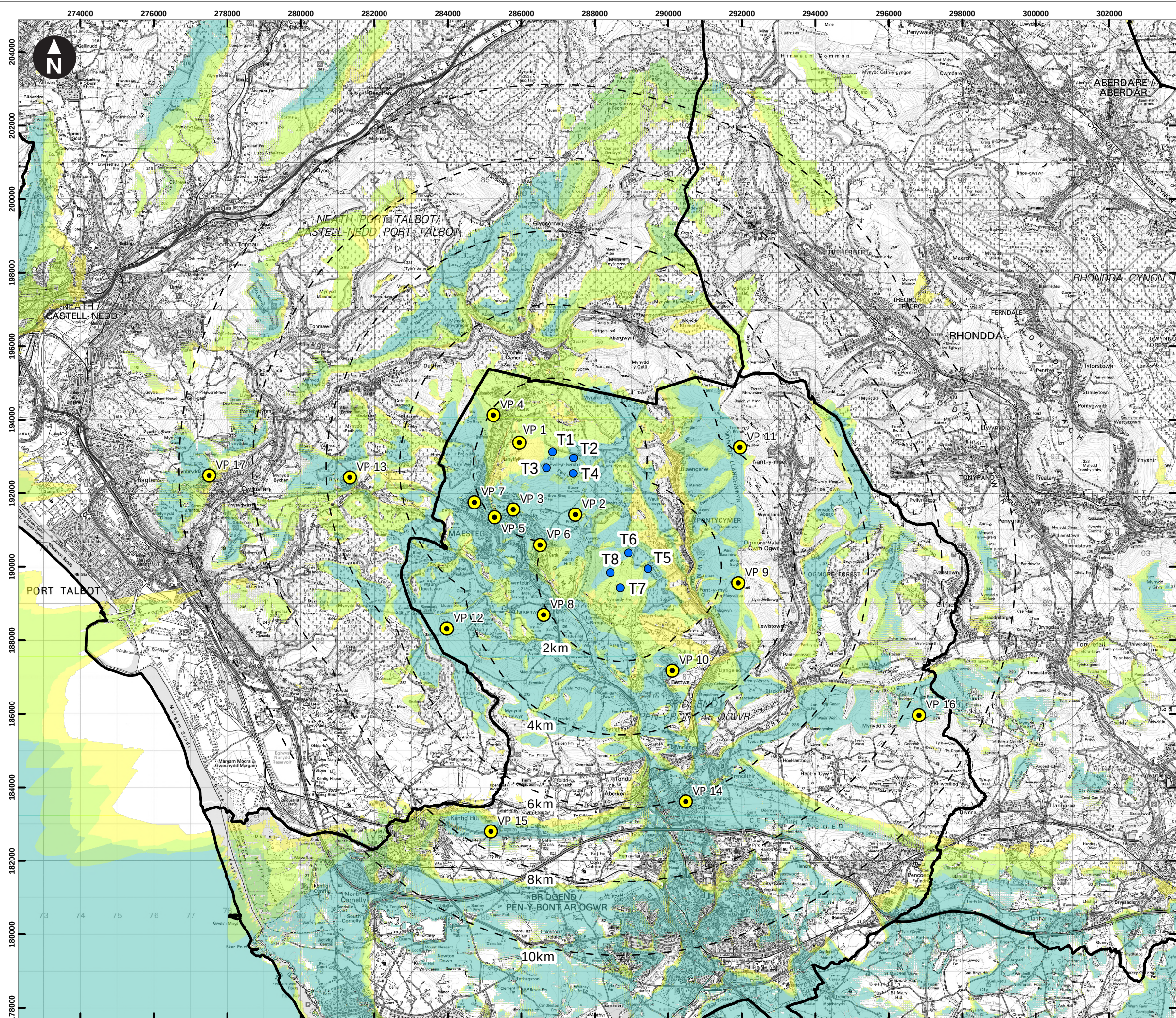
Figure 6.4 Detailed Zone of Theoretical Visibility (ZTV) to Blade Tip with Viewpoint Locations
