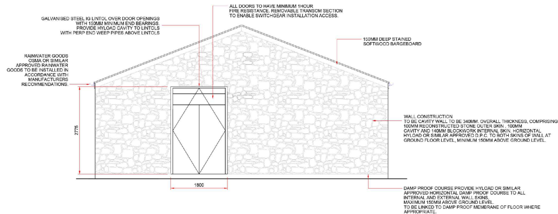
PROPOSED GABLE END (LEFT) ELEVATION
