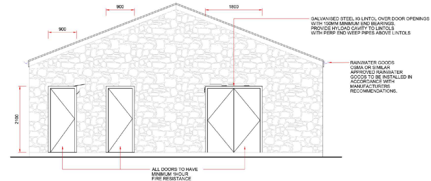
PROPOSED GABLE END (RIGHT) ELEVATION
