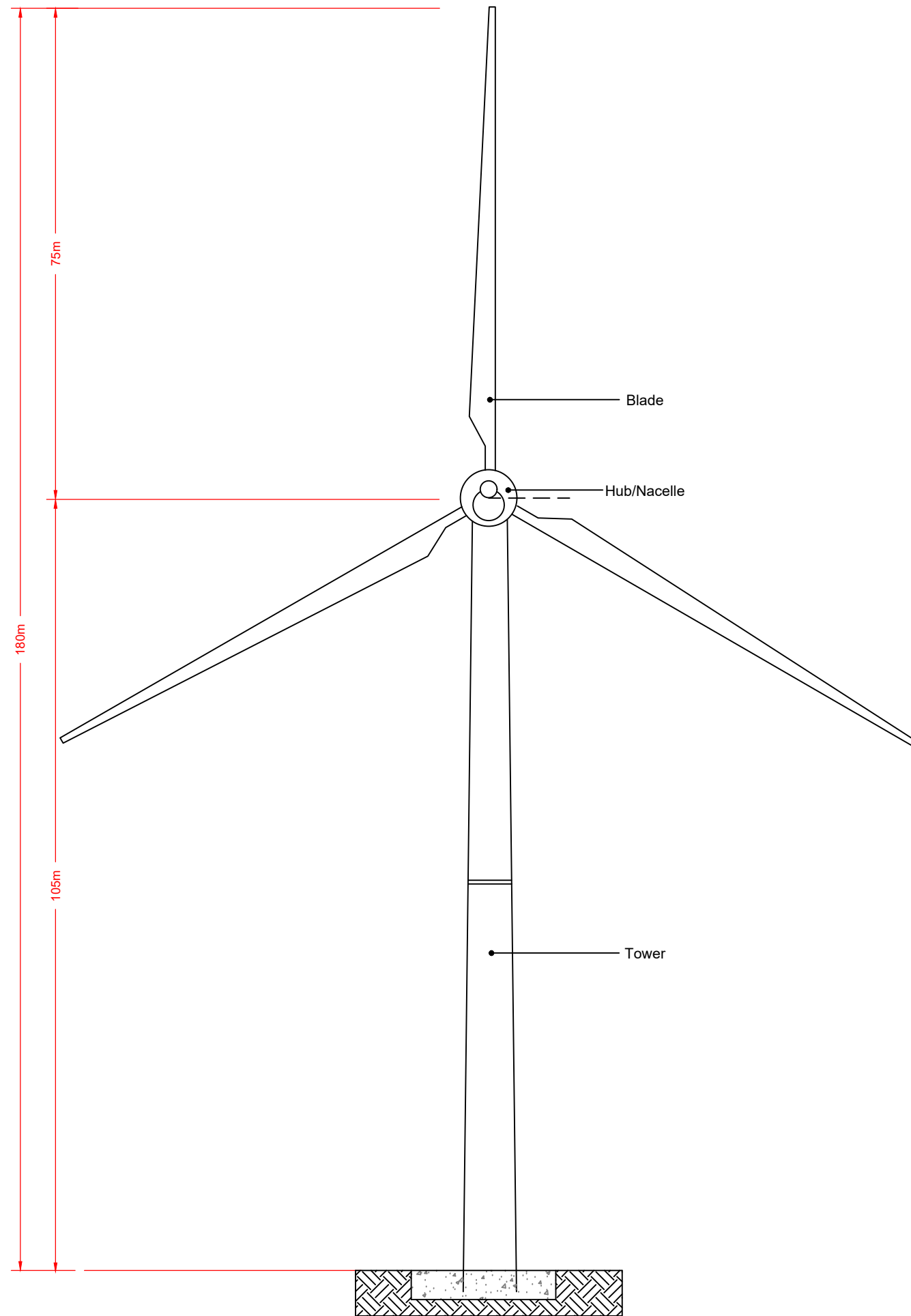
Figure 4.2 Typical wind turbine with a tip height of 180m
