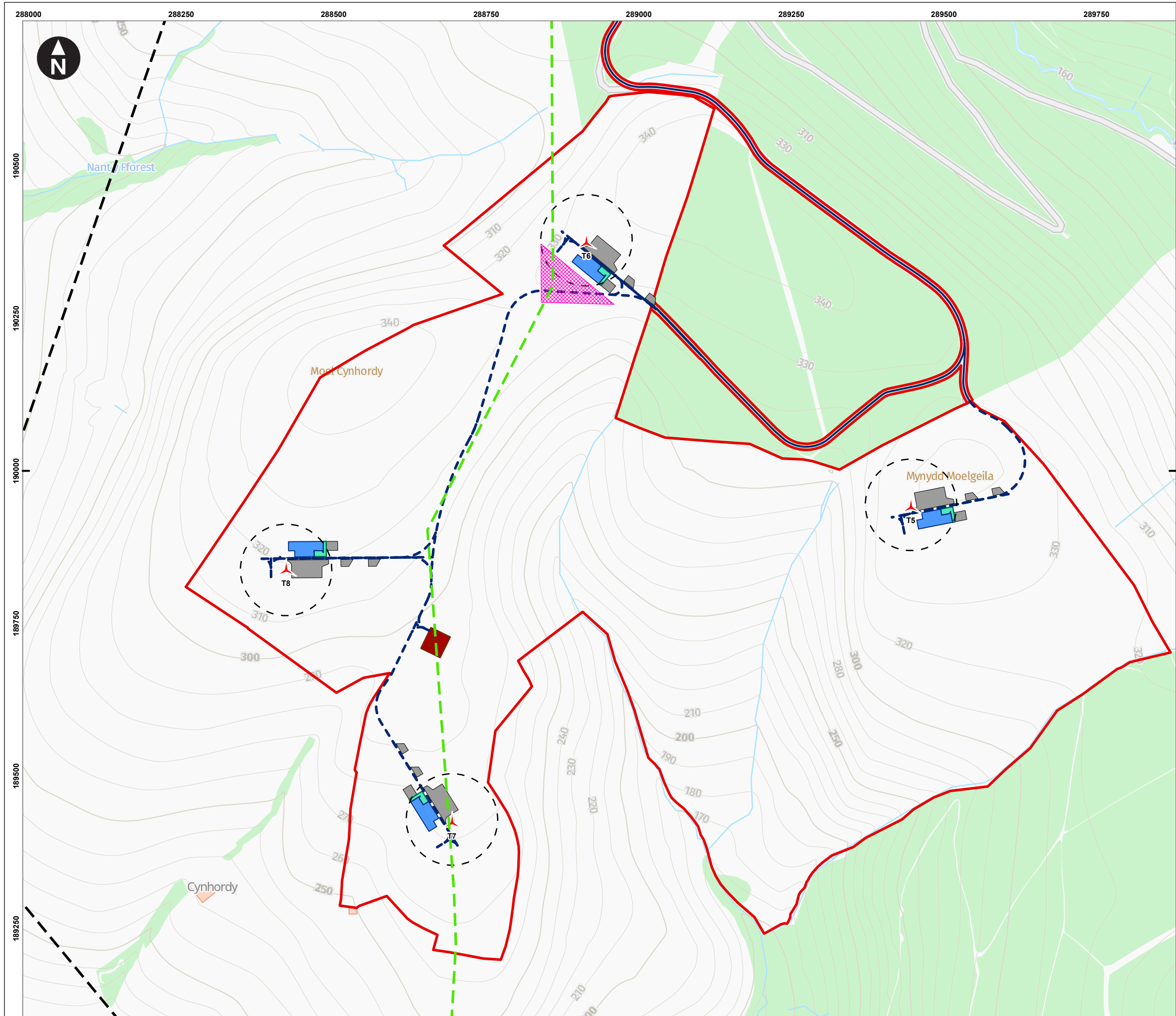
Figure 1.4 Southern array site layout
